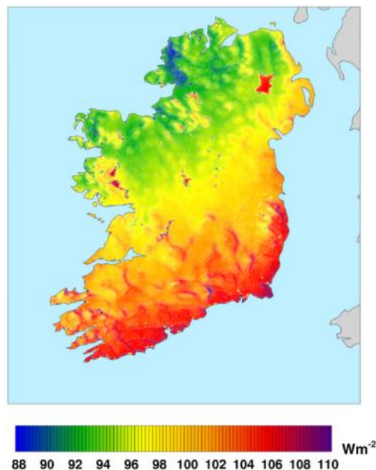
Figure 8: Average surface radiation for the period 1981 – 2000
